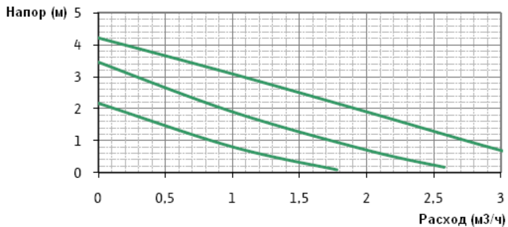
Wilo RS 25/4-3
